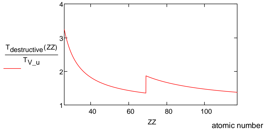
Figure 1. Destructive Thermal Limit
